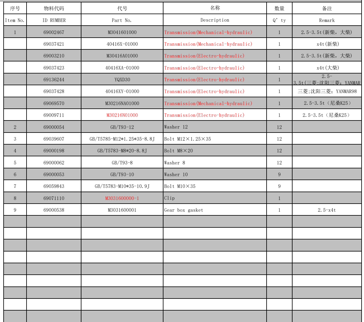
传动装置安装(液力式)/DRIVE UNIT ASS'Y (TOR-CON TYPE)
