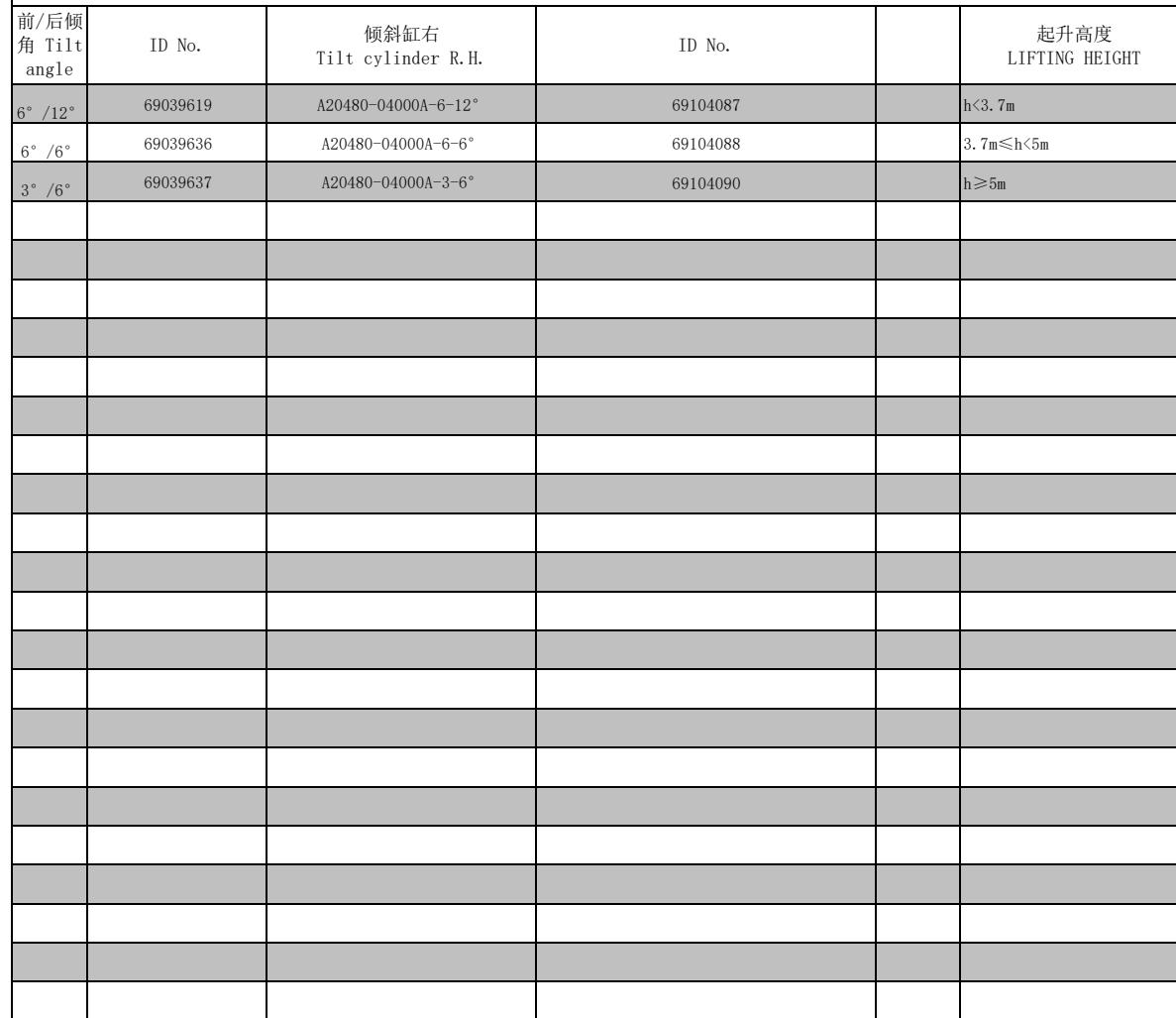
倾斜油缸(2.5t)/TILT CYLINDER(2.5t)
